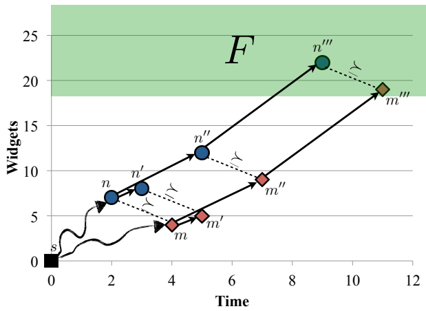
Figure 2: Abstract representation of search with compatible partial orders. The shaded area represents the goal region. Both m and n are reachable from the start state. Because n is a better state than m , and n 's successors “stay ahead” of m 's, we can safely avoid expanding m while still preserving optimality.
