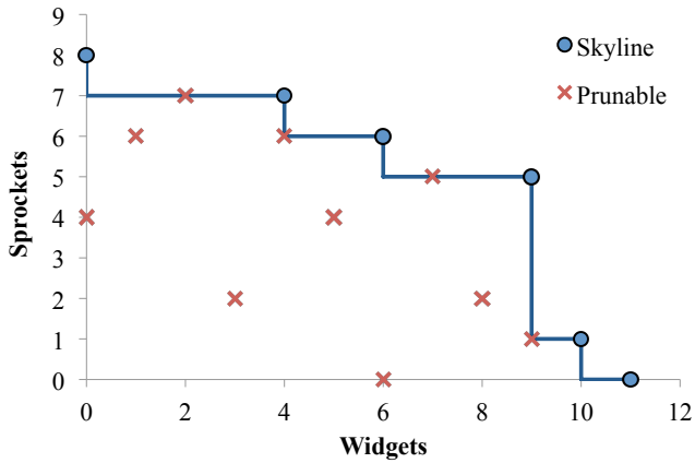
Figure 1: An example set of states in a two-resource planning domain. If all pictured states have the same cost, then only those shown as circles are worth exploring; the X’s can be safely pruned.
